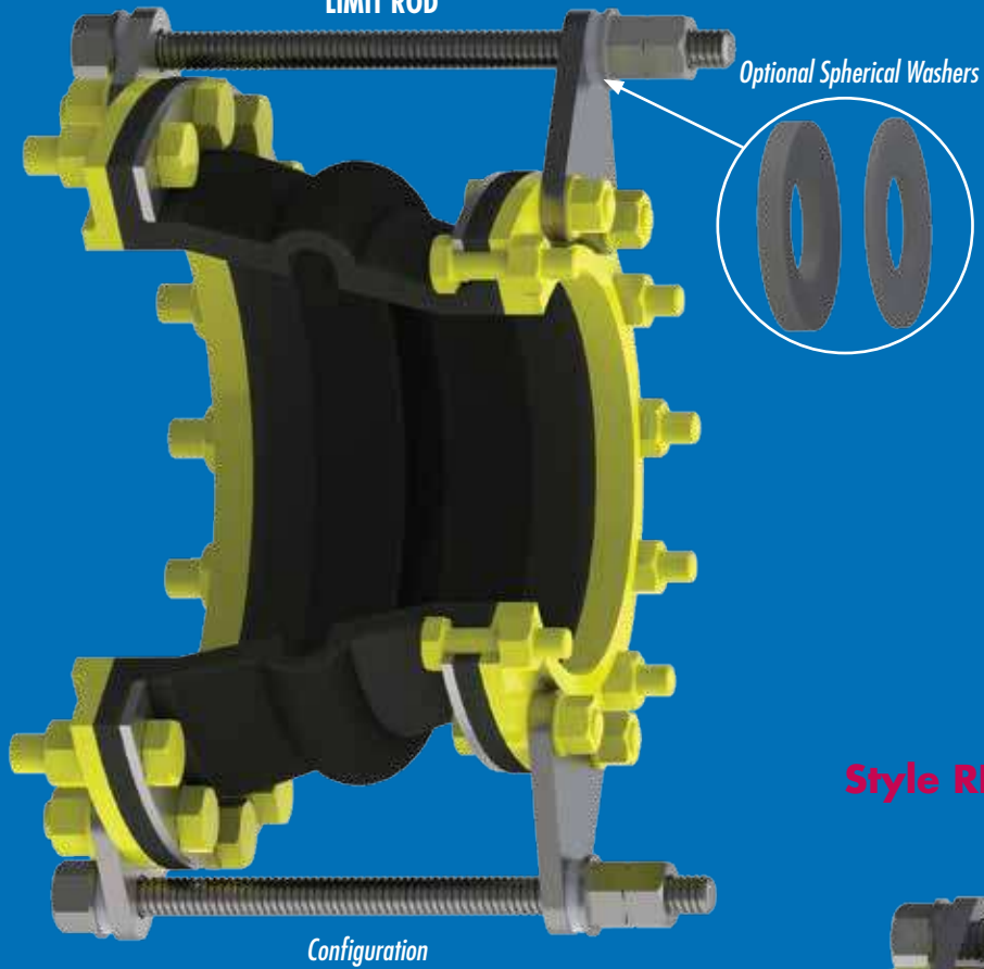
Figure 1 LIMIT ROD
