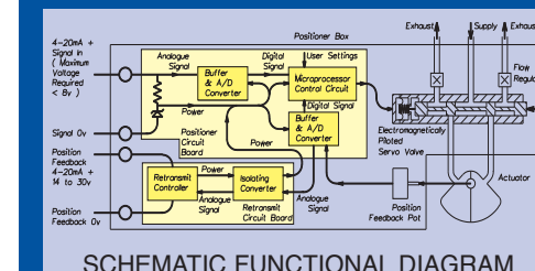
SCHEMATIC FUNCTIONAL DIAGRAM
